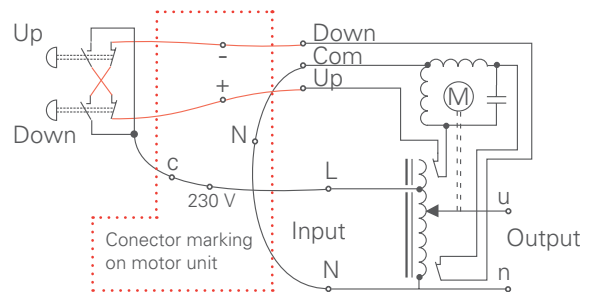
Remote control application principle (230 V motor)
