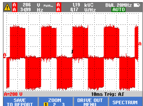
Drive output waveform with auto triggering
