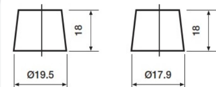
Positive Terminal
